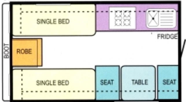
SPRINTER P 120 x 70 - 1
